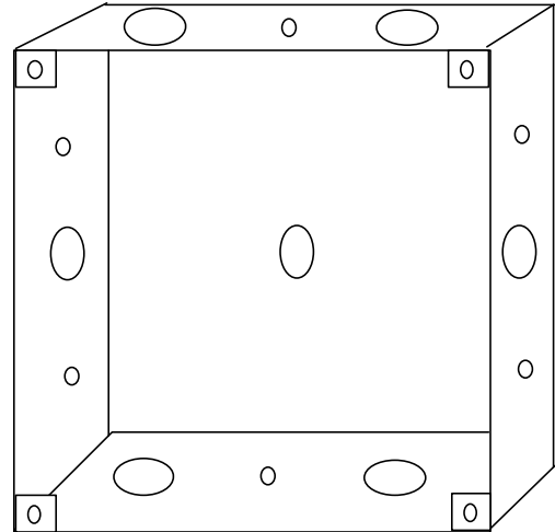
ADA 100 5 Zone Master Station & Area Station Back Box 8" L x 8" W x 4" D
