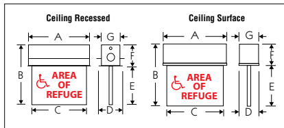
DIMENSIONS (in.)
